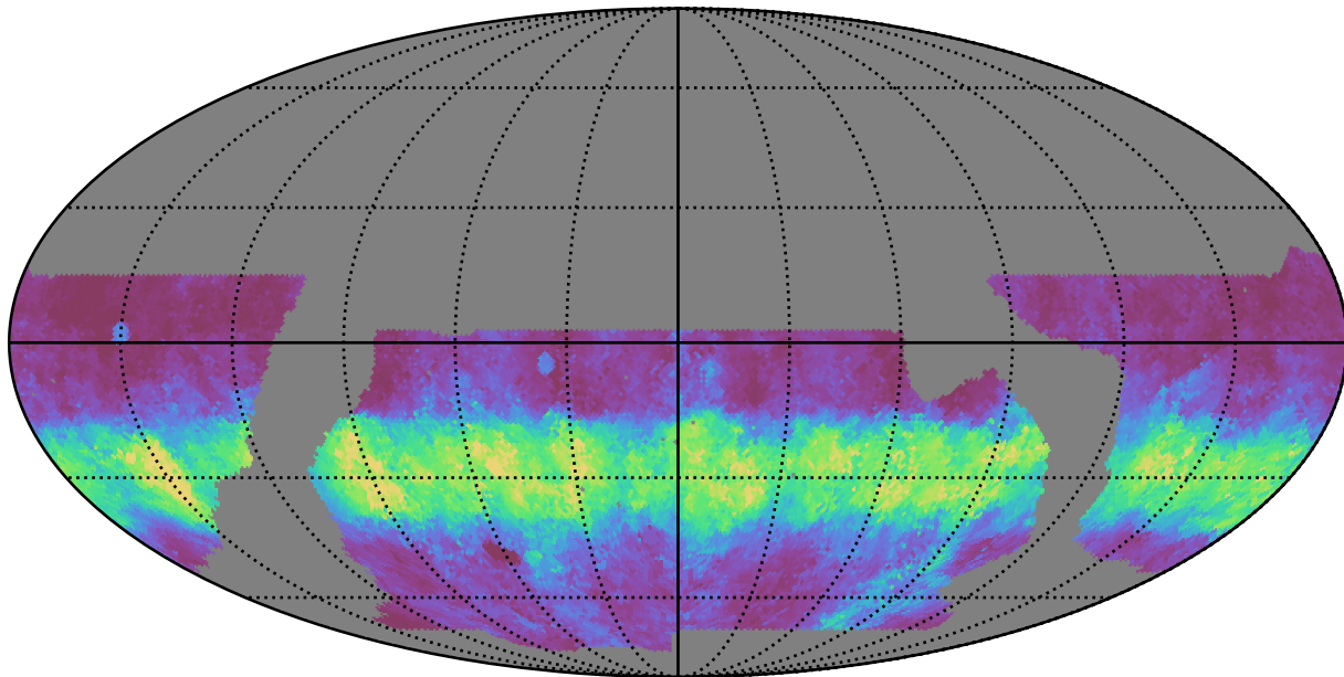
baseline_v2.1_10yrs WFD u band: Median normairmass
