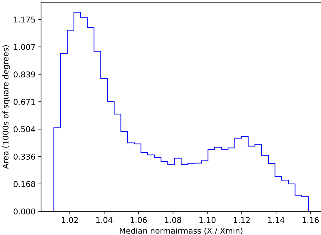
baseline_v2.1_10yrs WFD u band: Median normairmass
