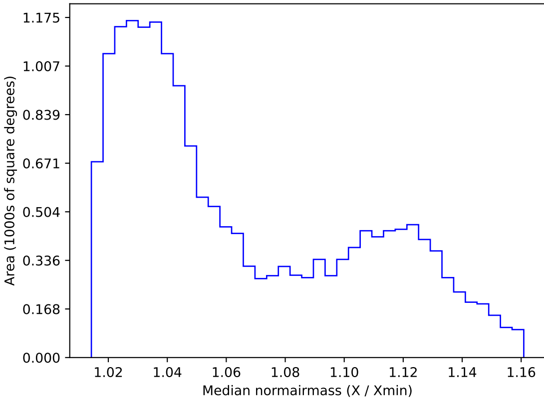
baseline_v2.1_10yrs WFD r band: Median normairmass
