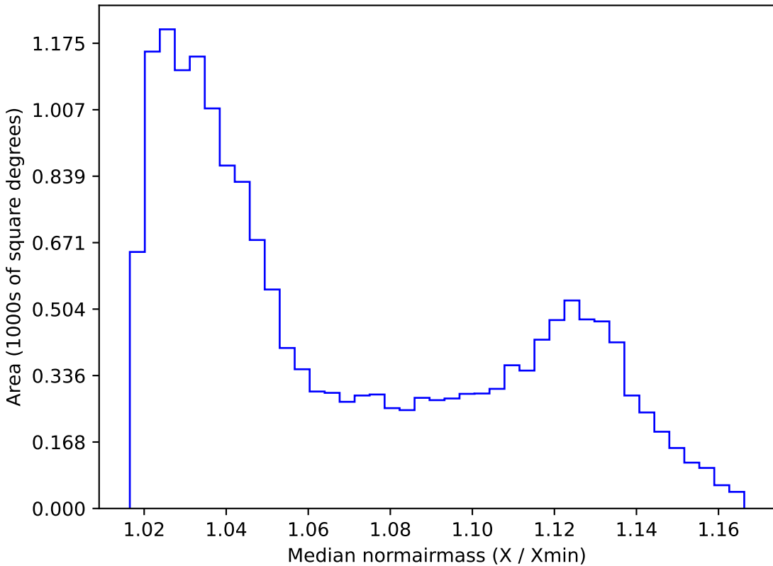
baseline_v2.1_10yrs WFD i band: Median normairmass
