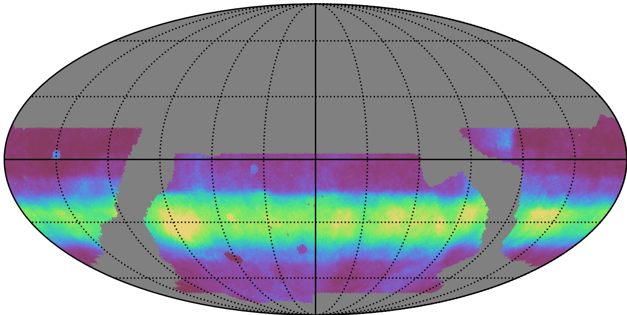
baseline_v2.1_10yrs WFD all bands: Median normairmass
