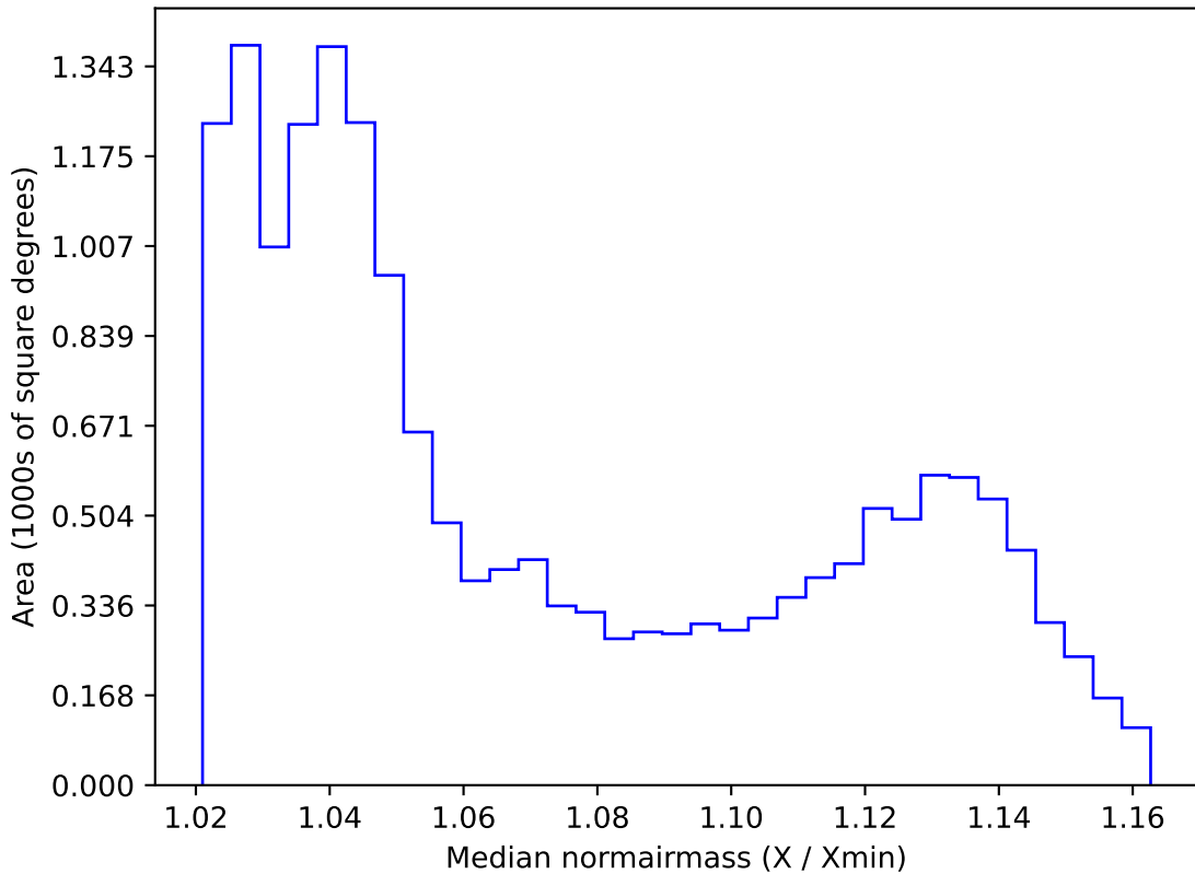
baseline_v2.1_10yrs WFD all bands: Median normairmass
