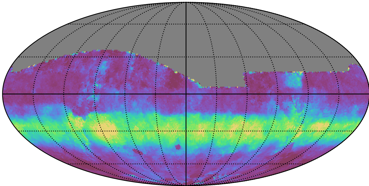
baseline_v2.1_10yrs All sky z band: Median normairmass
