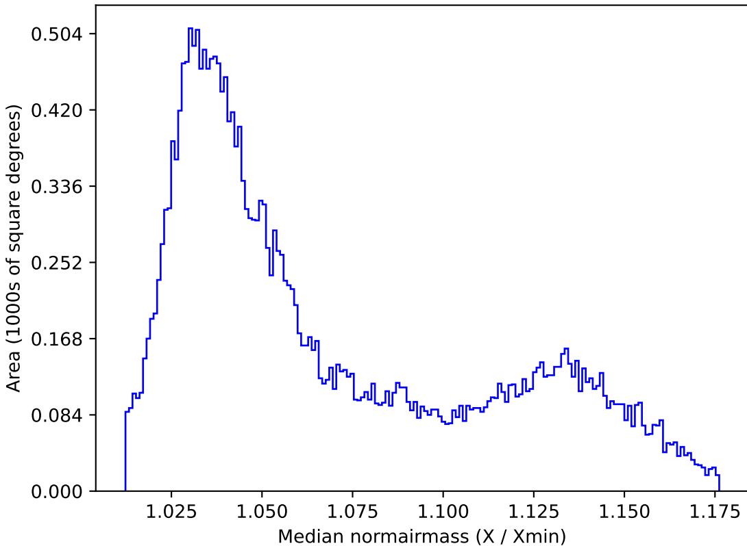
baseline_v2.1_10yrs All sky z band: Median normairmass
