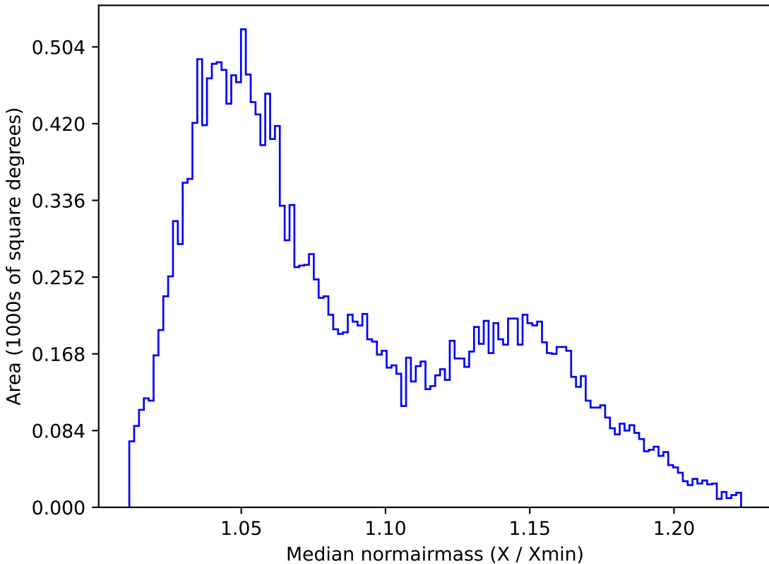
baseline_v2.1_10yrs All sky y band: Median normairmass
