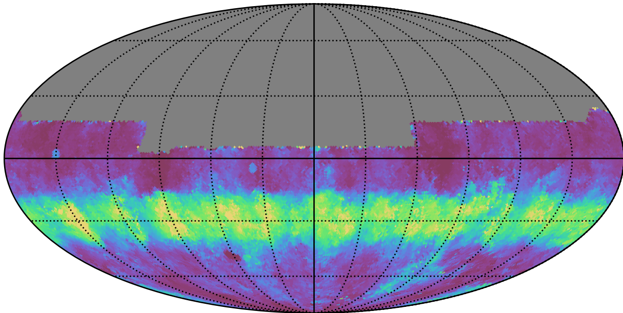
baseline_v2.1_10yrs All sky u band: Median normairmass
