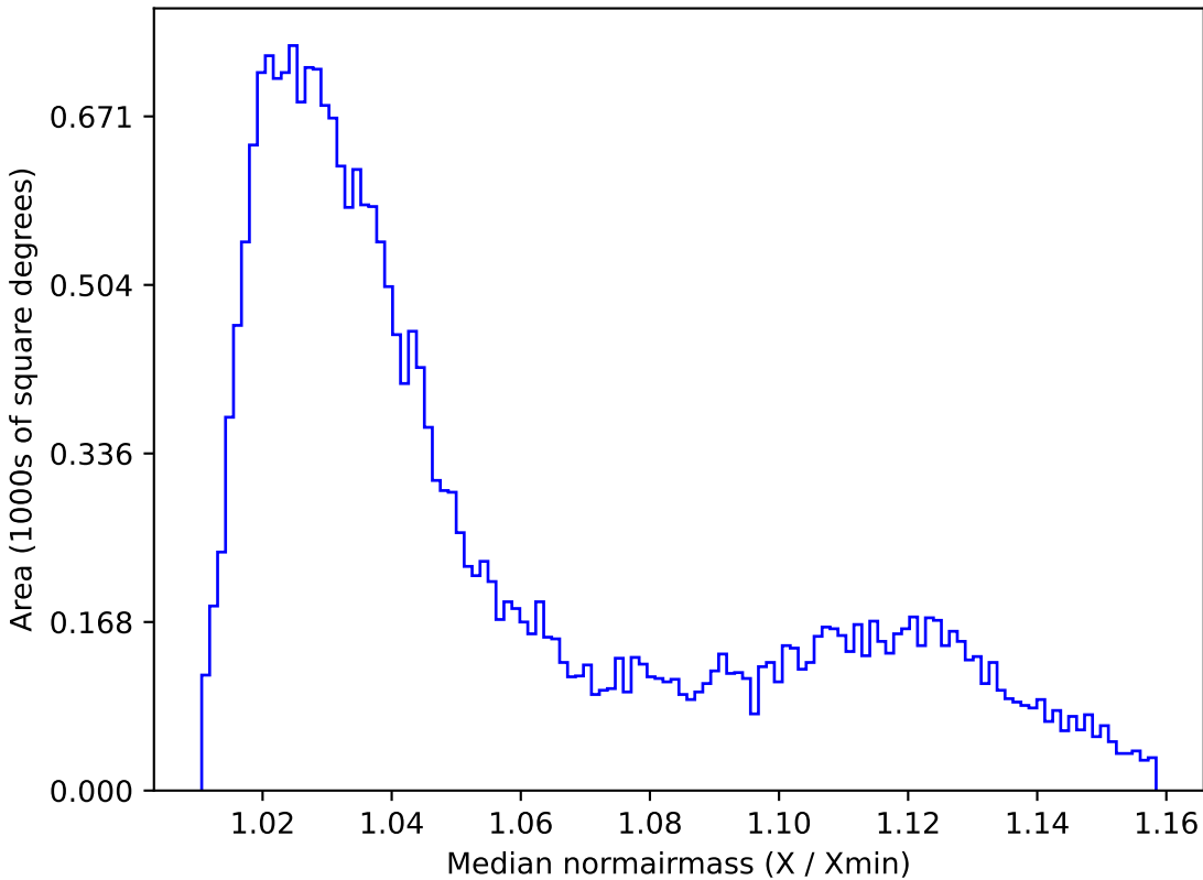
baseline_v2.1_10yrs All sky r band: Median normairmass
