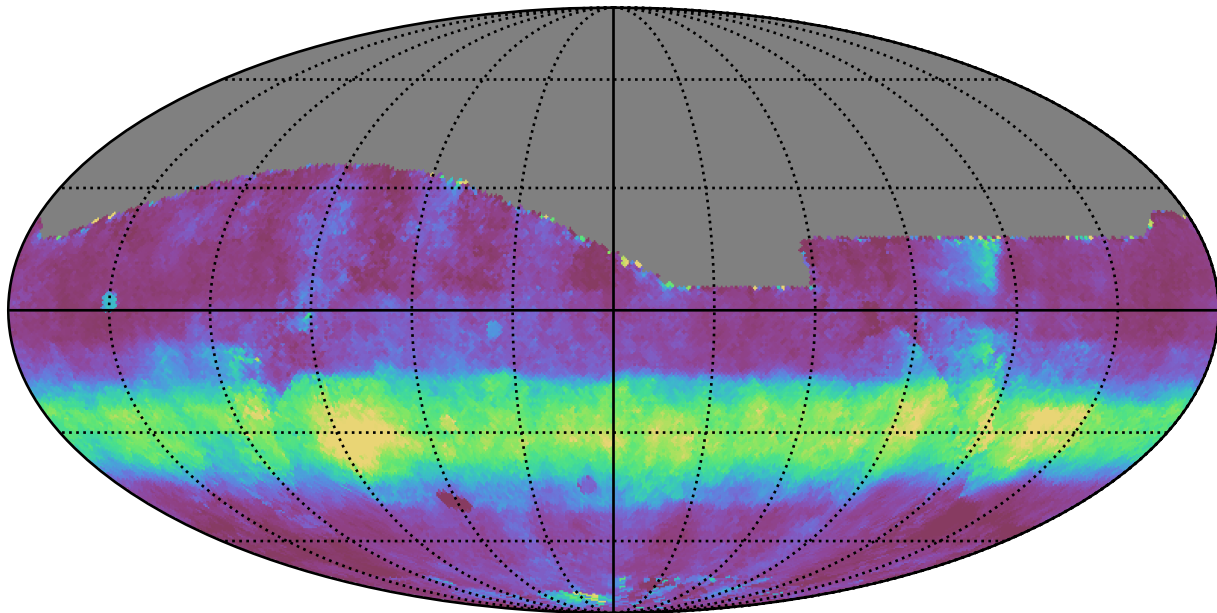
baseline_v2.1_10yrs All sky i band: Median normairmass
