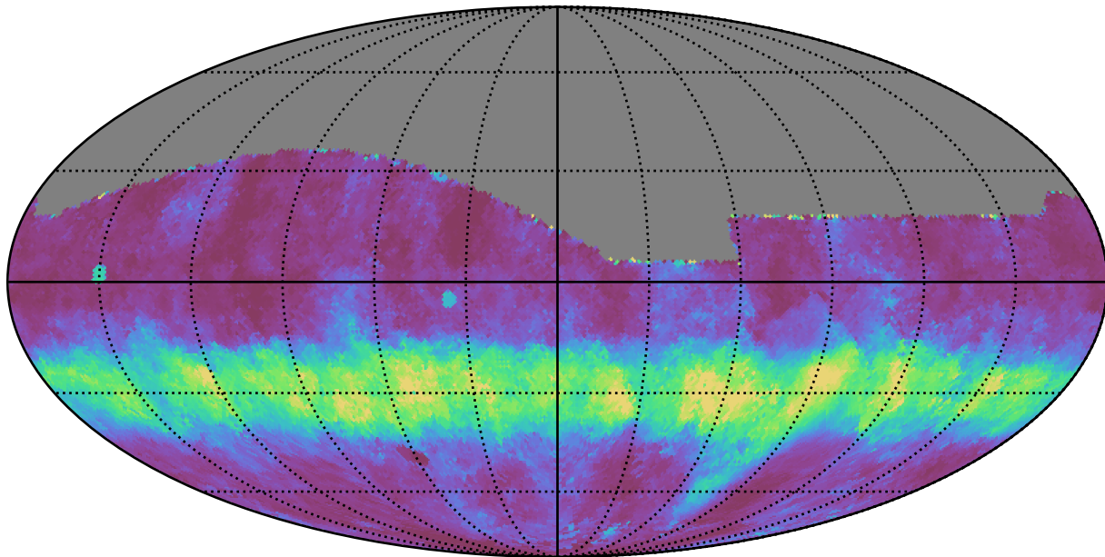
baseline_v2.1_10yrs All sky g band: Median normairmass
