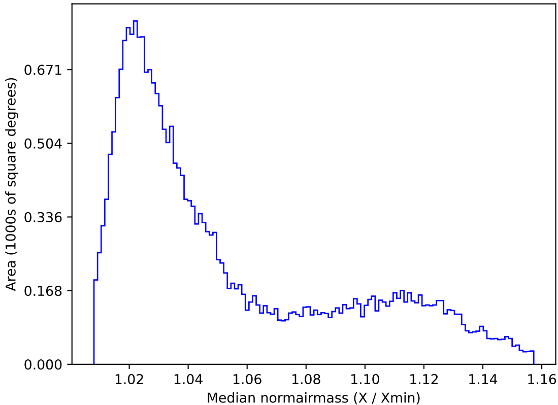
baseline_v2.1_10yrs All sky g band: Median normairmass
