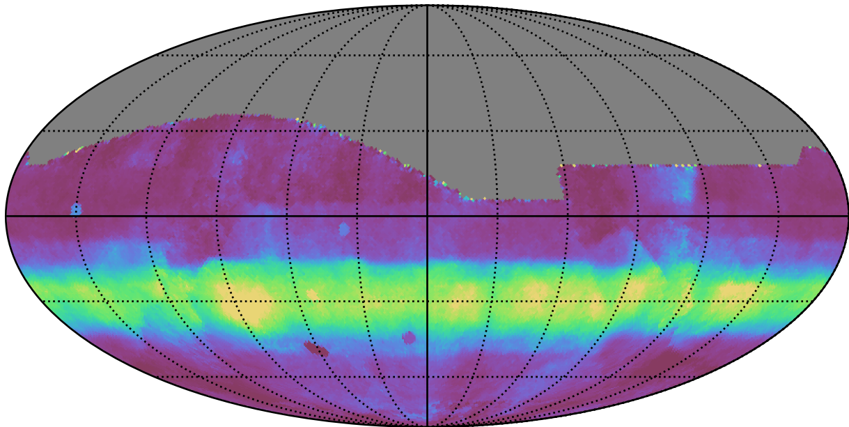
baseline_v2.1_10yrs All sky all bands: Median normairmass
