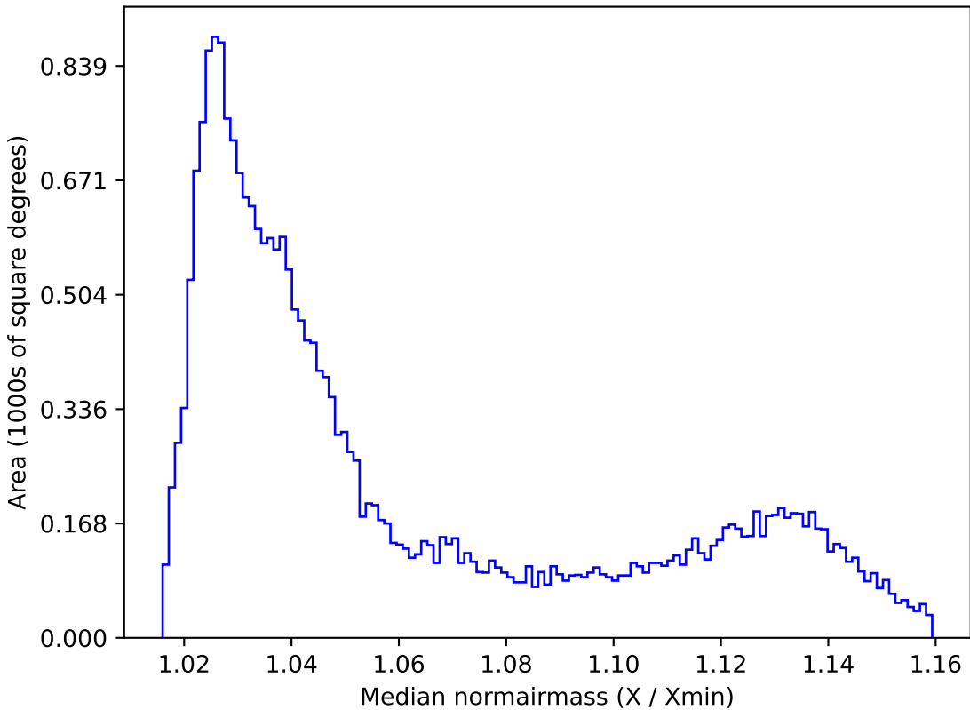
baseline_v2.1_10yrs All sky all bands: Median normairmass
