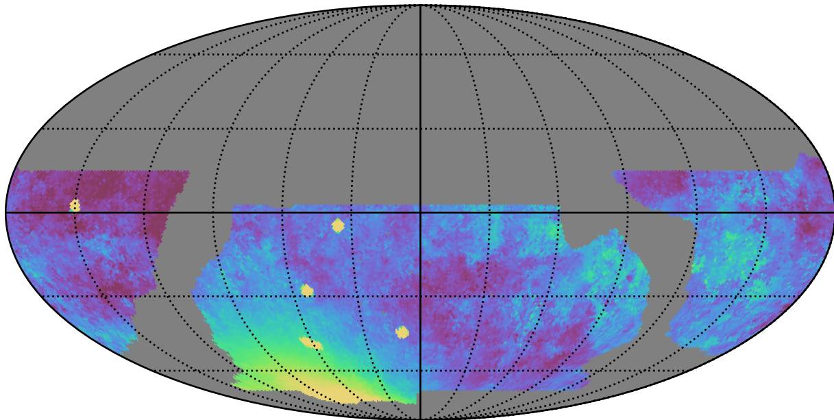
baseline_v2.1_10yrs WFD z band: Median moonDistance
