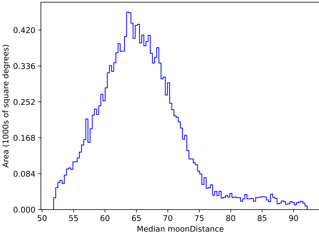
baseline_v2.1_10yrs WFD z band: Median moonDistance
