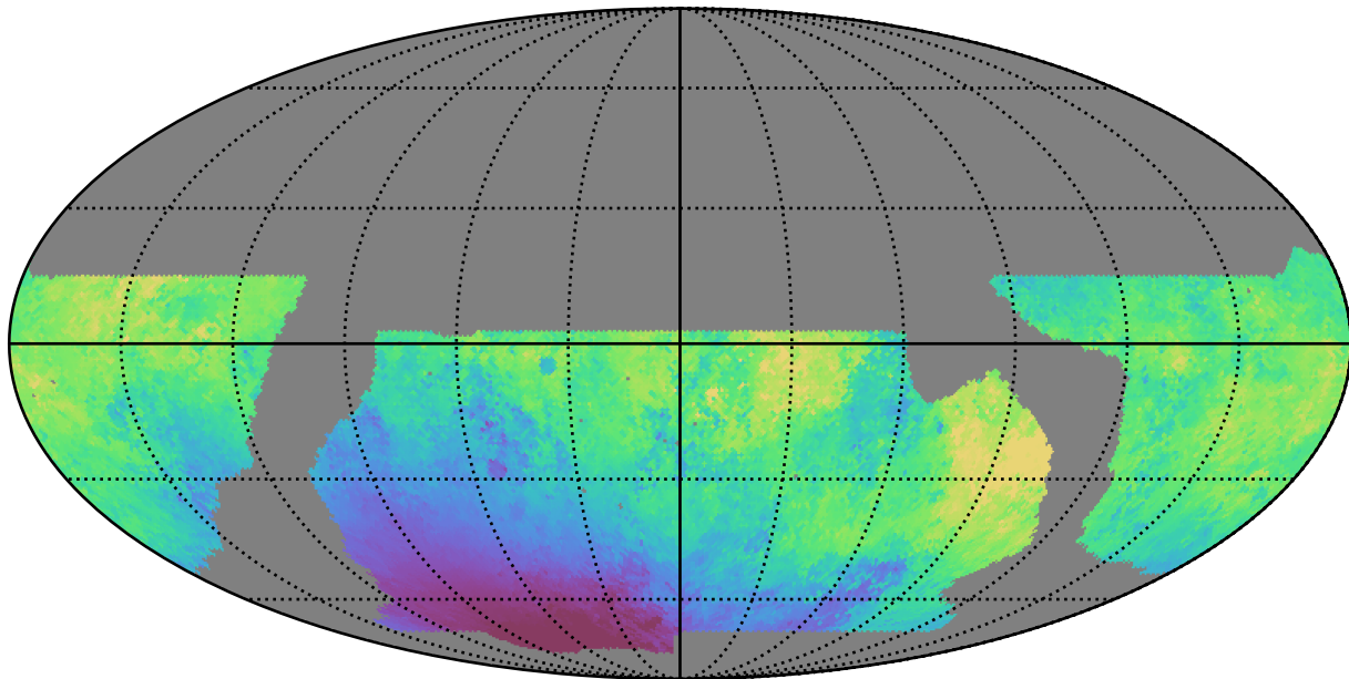
baseline_v2.1_10yrs WFD u band: Median moonDistance
