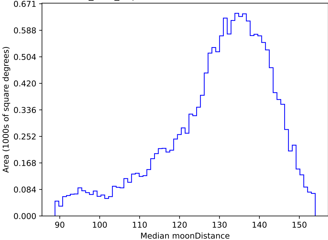
baseline_v2.1_10yrs WFD u band: Median moonDistance
