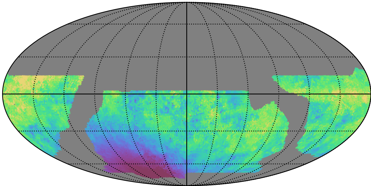
baseline_v2.1_10yrs WFD r band: Median moonDistance
