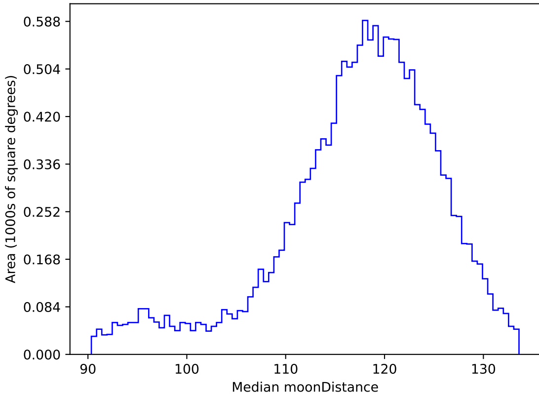
baseline_v2.1_10yrs WFD r band: Median moonDistance
