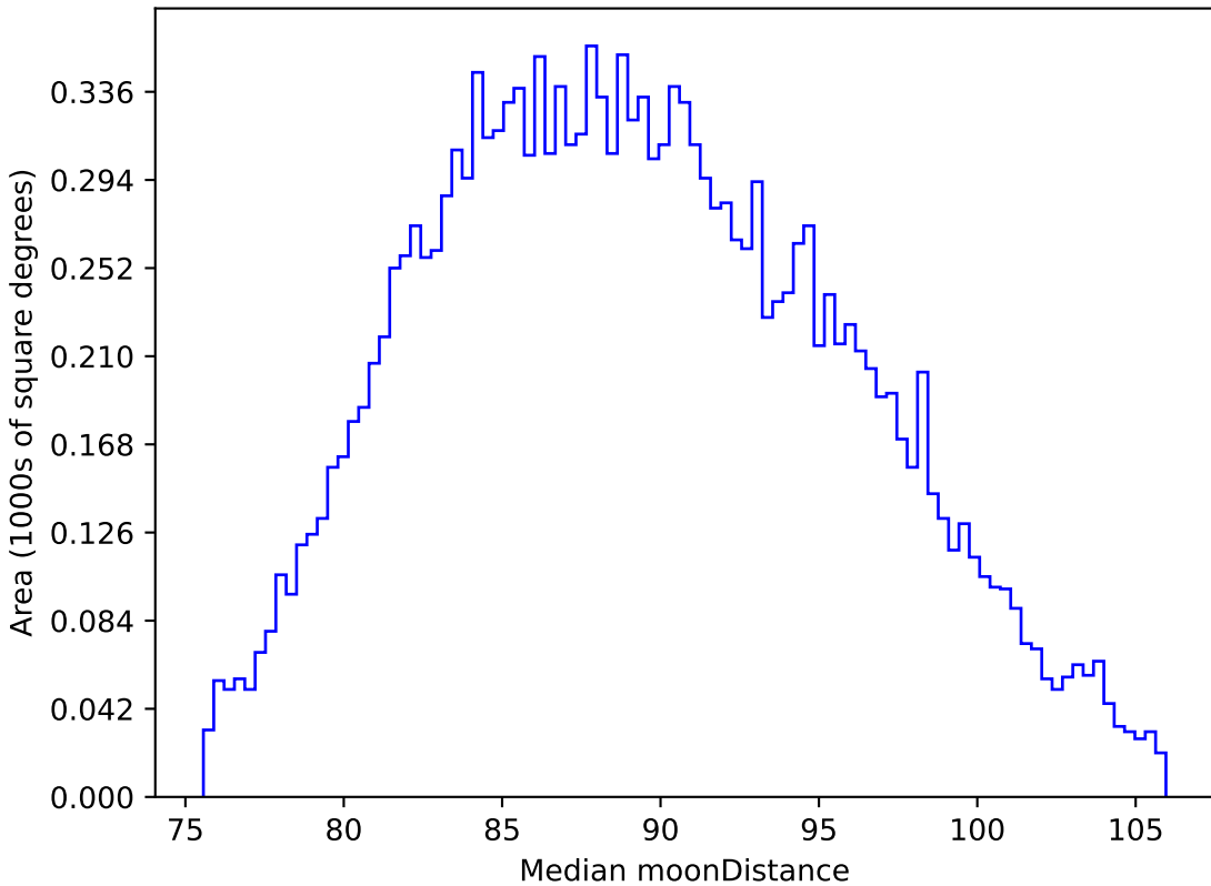
baseline_v2.1_10yrs WFD i band: Median moonDistance
