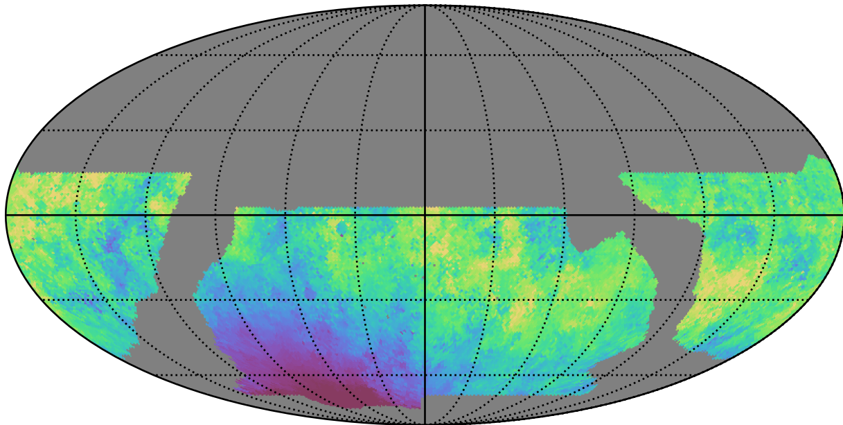
baseline_v2.1_10yrs WFD g band: Median moonDistance
