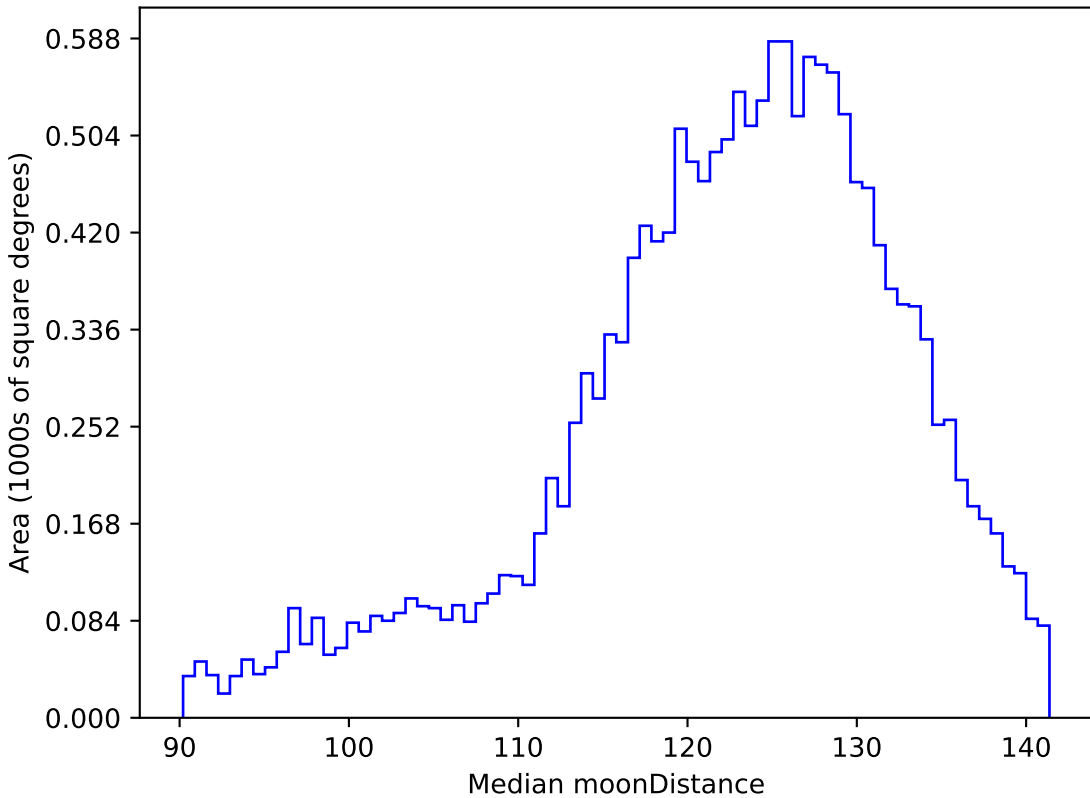
baseline_v2.1_10yrs WFD g band: Median moonDistance
