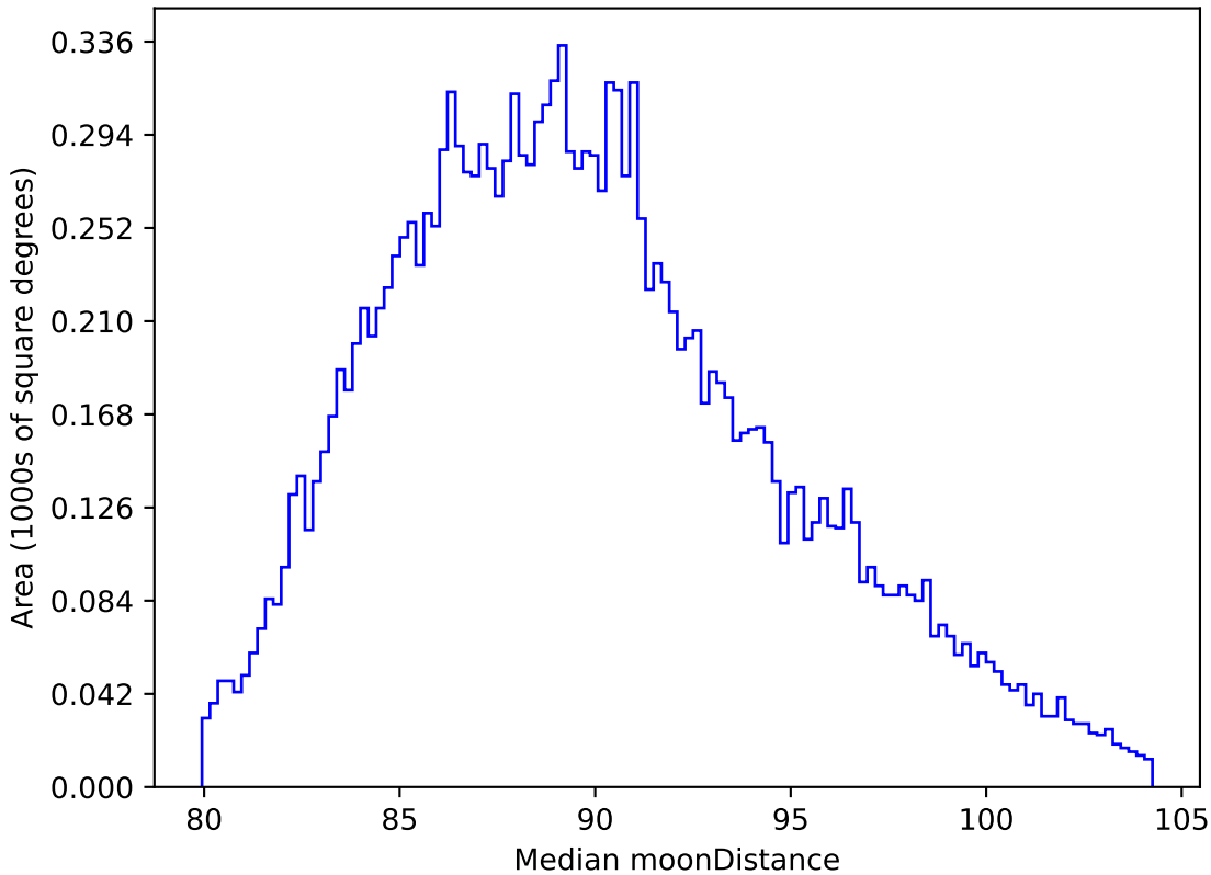
baseline_v2.1_10yrs WFD all bands: Median moonDistance
