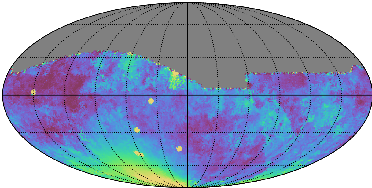
baseline_v2.1_10yrs All sky z band: Median moonDistance
