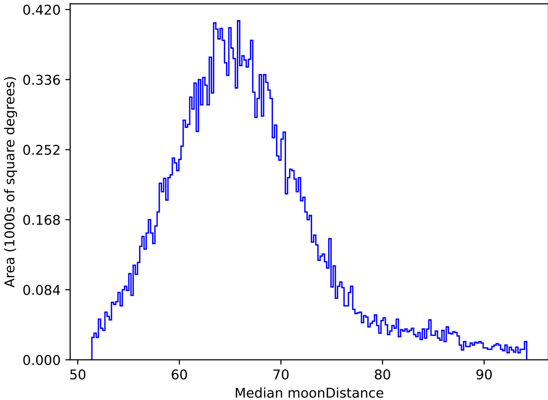
baseline_v2.1_10yrs All sky z band: Median moonDistance
