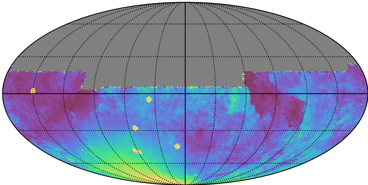
baseline_v2.1_10yrs All sky y band: Median moonDistance
