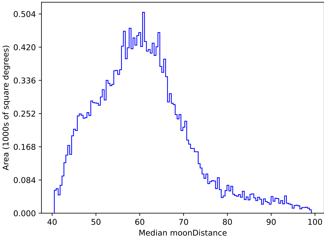
baseline_v2.1_10yrs All sky y band: Median moonDistance
