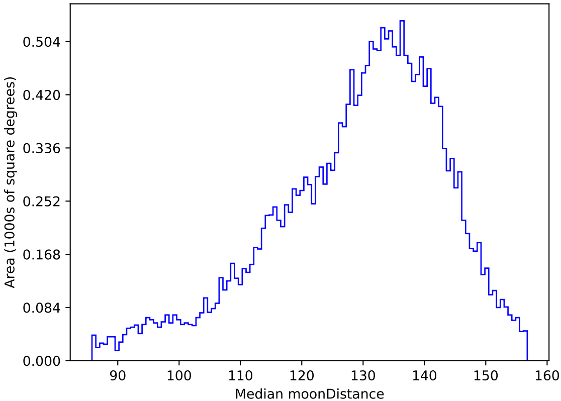
baseline_v2.1_10yrs All sky u band: Median moonDistance
