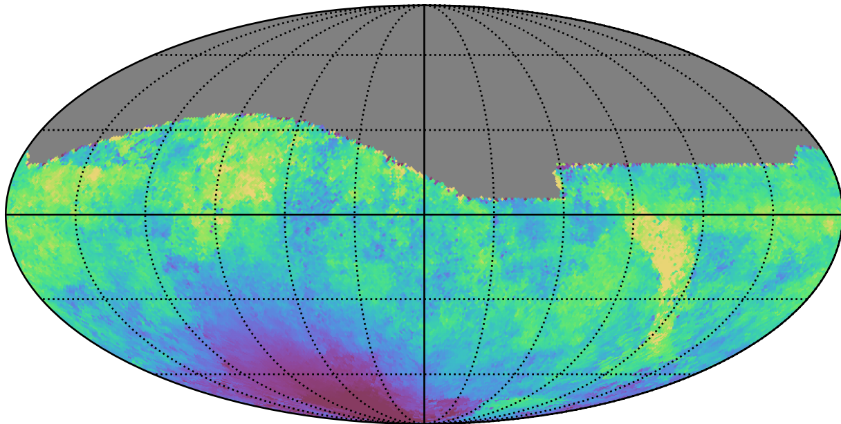
baseline_v2.1_10yrs All sky r band: Median moonDistance
