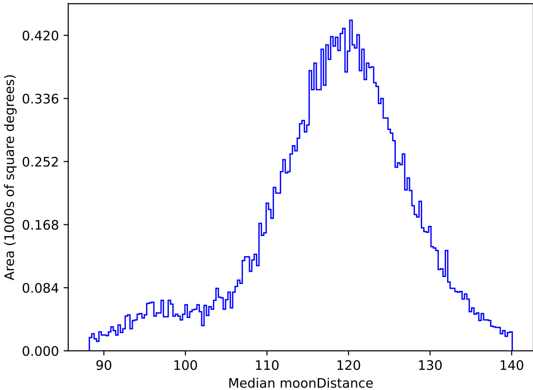
baseline_v2.1_10yrs All sky r band: Median moonDistance
