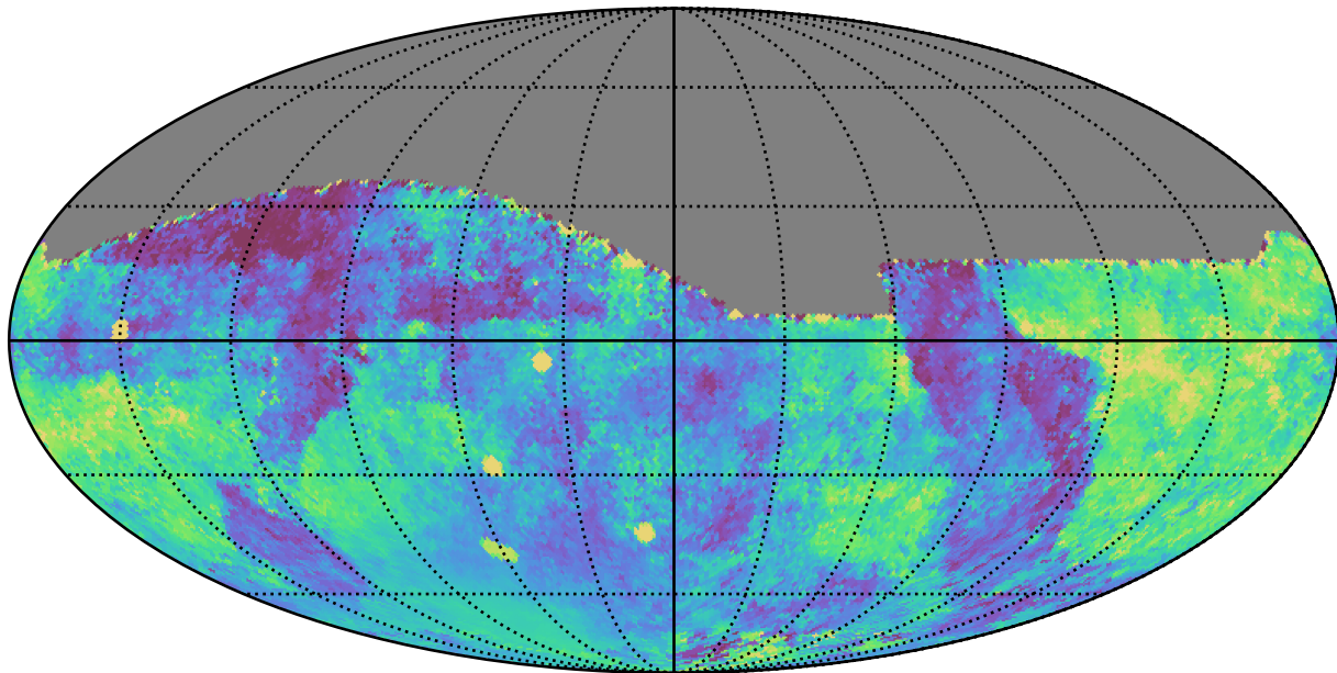
baseline_v2.1_10yrs All sky i band: Median moonDistance
