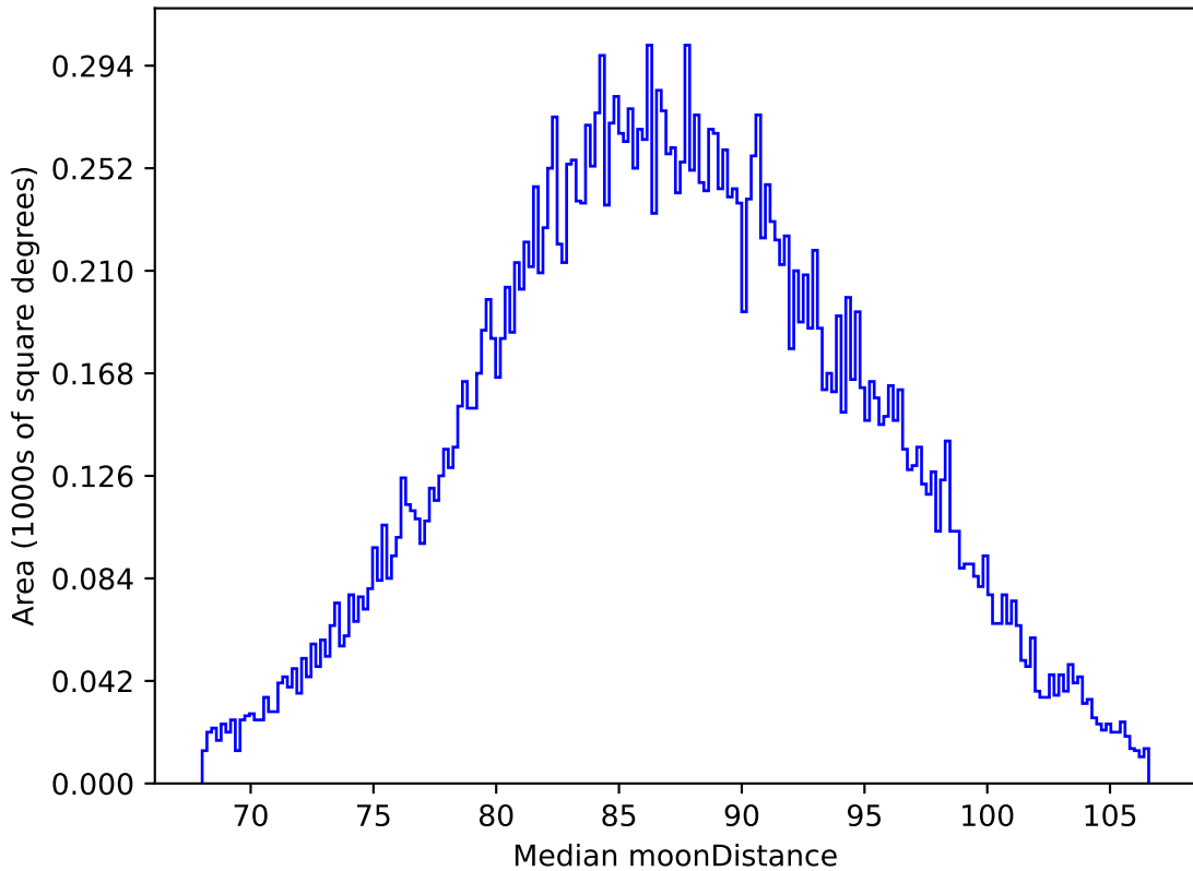
baseline_v2.1_10yrs All sky i band: Median moonDistance
