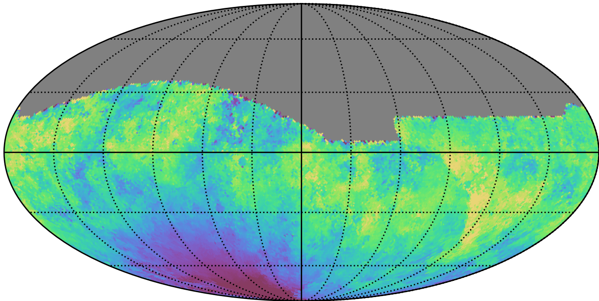
baseline_v2.1_10yrs All sky g band: Median moonDistance
