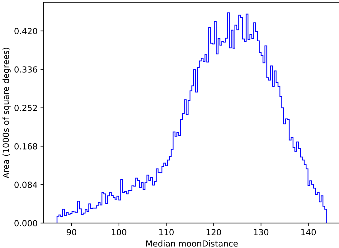
baseline_v2.1_10yrs All sky g band: Median moonDistance
