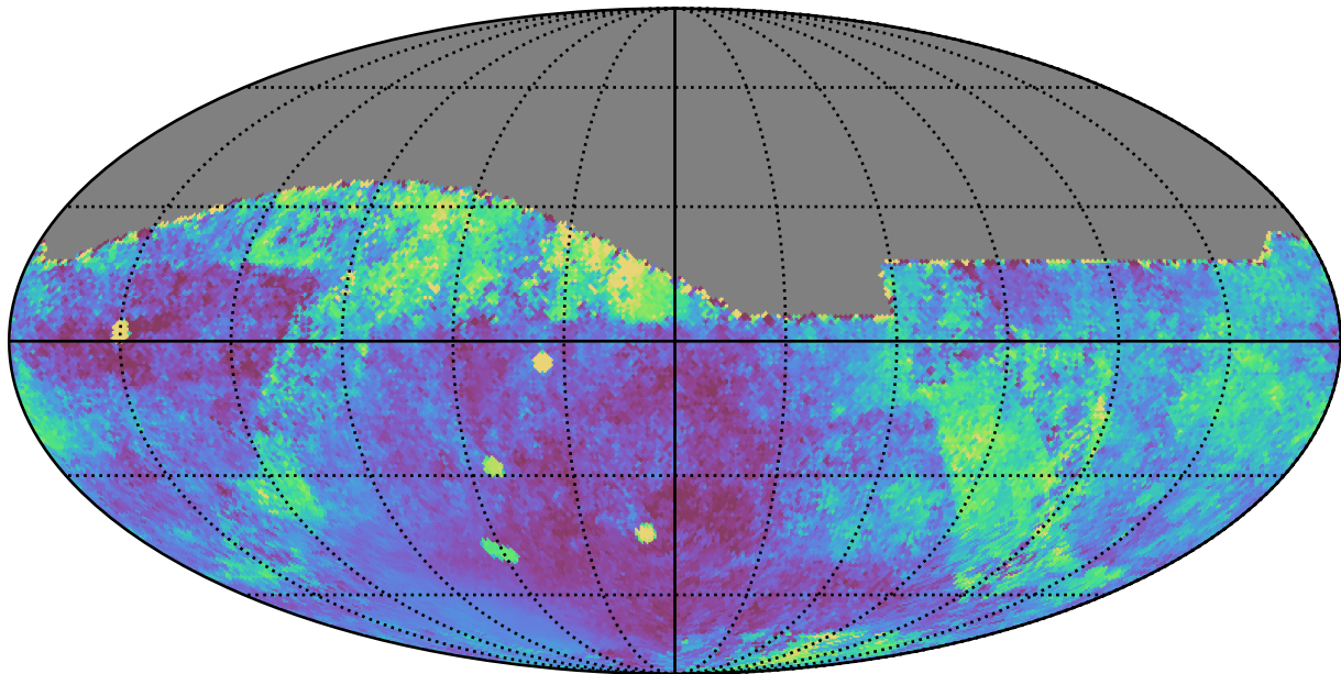
baseline_v2.1_10yrs All sky all bands: Median moonDistance
