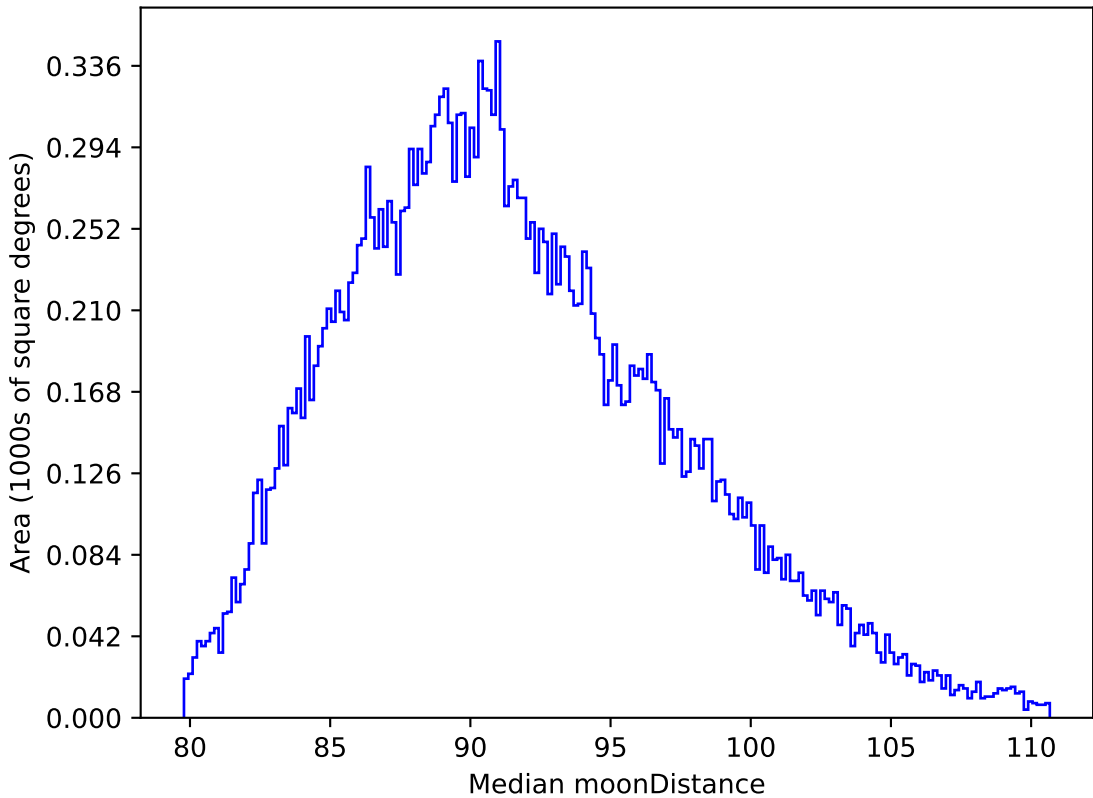
baseline_v2.1_10yrs All sky all bands: Median moonDistance
