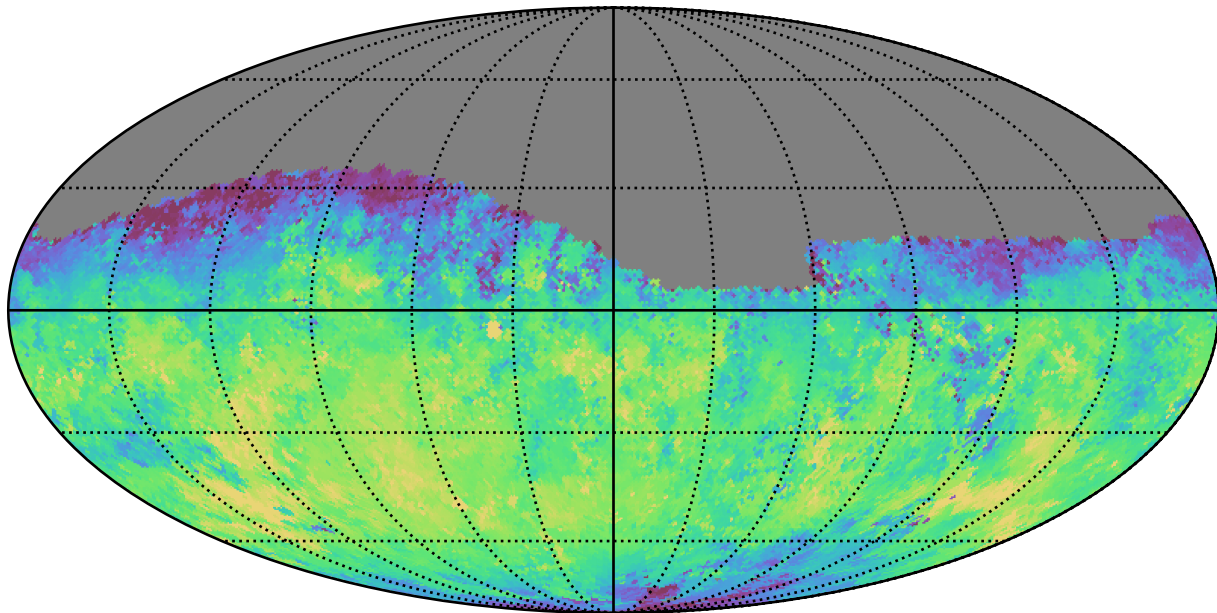
baseline_v2.1_10yrs Yr 1 z band: Median fiveSigmaDepth
