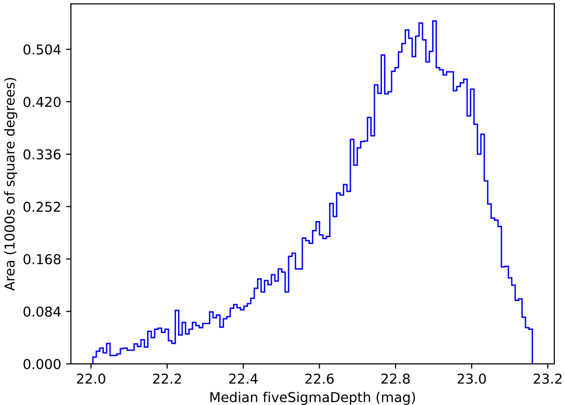
baseline_v2.1_10yrs Yr 1 z band: Median fiveSigmaDepth
