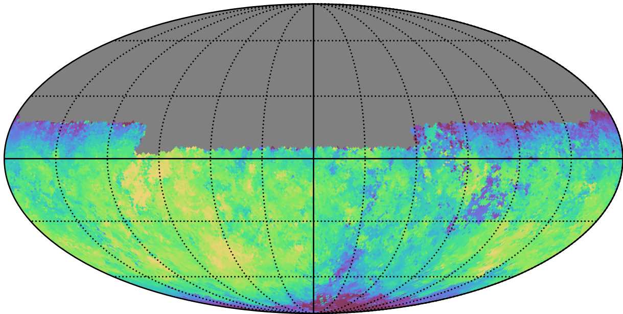
baseline_v2.1_10yrs Yr 1 y band: Median fiveSigmaDepth
