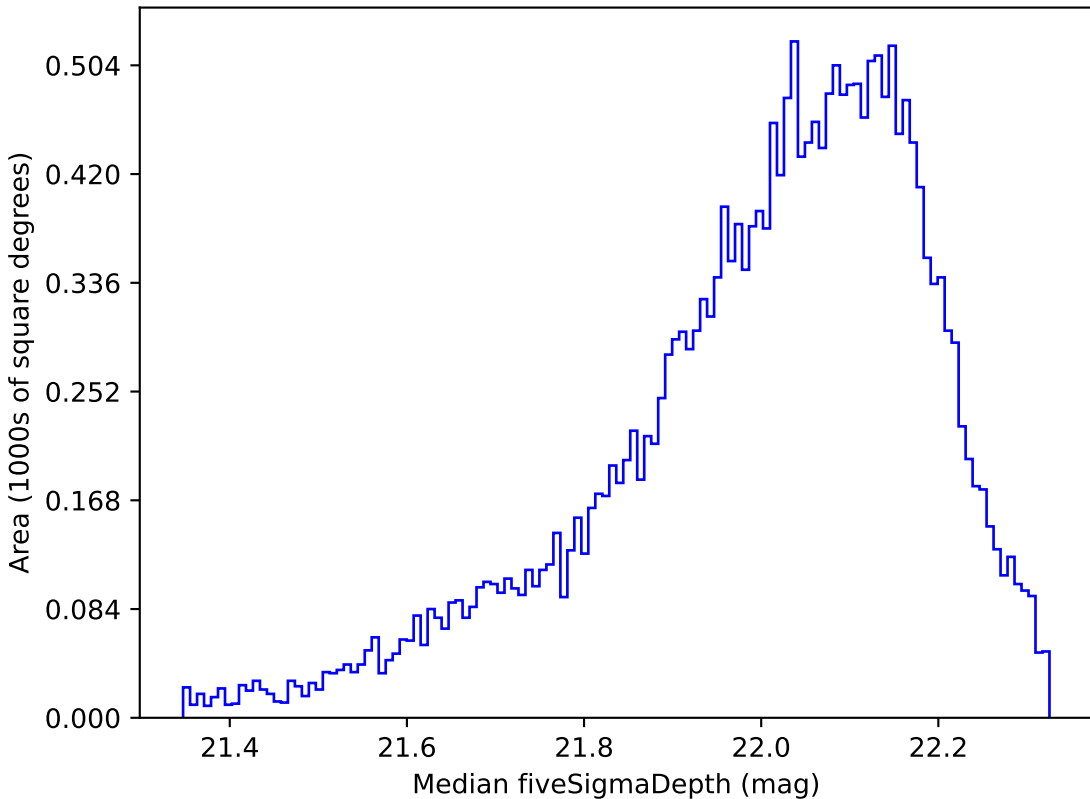
baseline_v2.1_10yrs Yr 1 y band: Median fiveSigmaDepth
