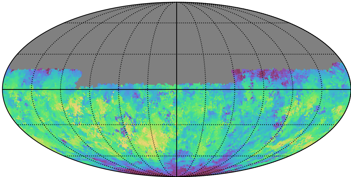
baseline_v2.1_10yrs Yr 1 u band: Median fiveSigmaDepth
