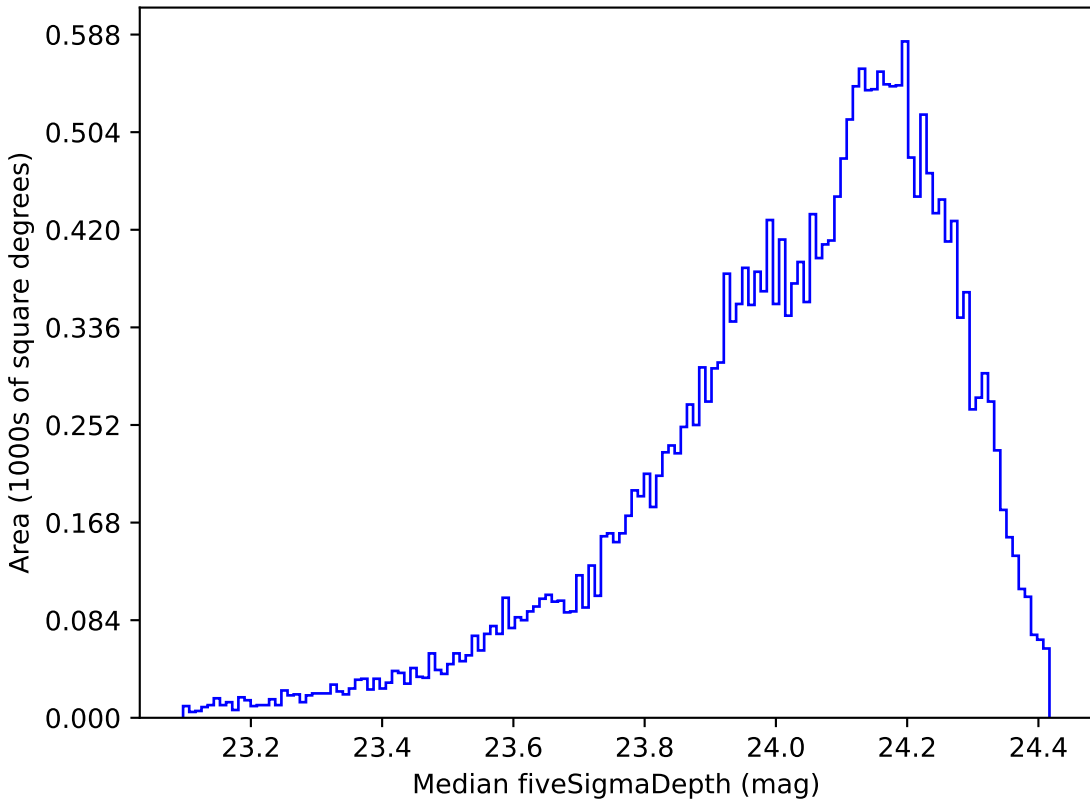
baseline_v2.1_10yrs Yr 1 r band: Median fiveSigmaDepth
