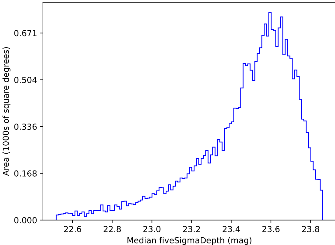
baseline_v2.1_10yrs Yr 1 i band: Median fiveSigmaDepth
