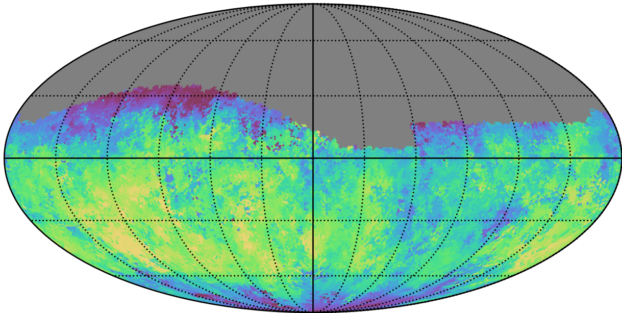
baseline_v2.1_10yrs Yr 1 g band: Median fiveSigmaDepth
