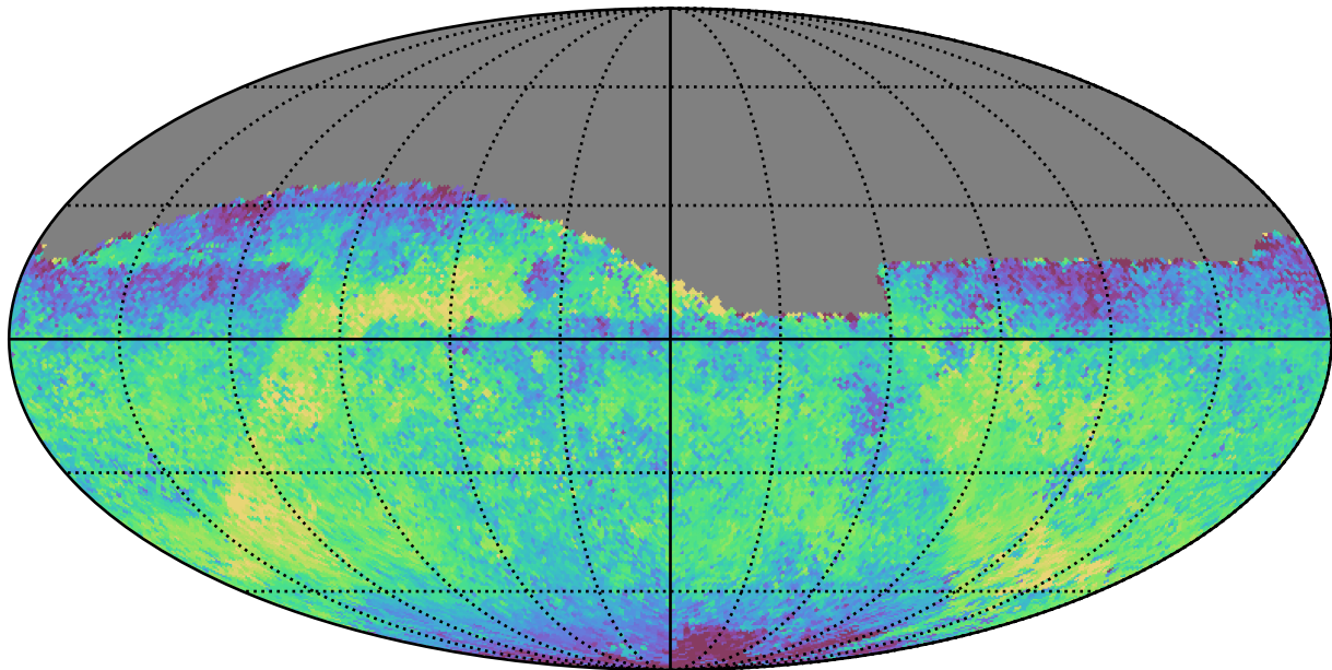
baseline_v2.1_10yrs Yr 1 all bands: Median fiveSigmaDepth
