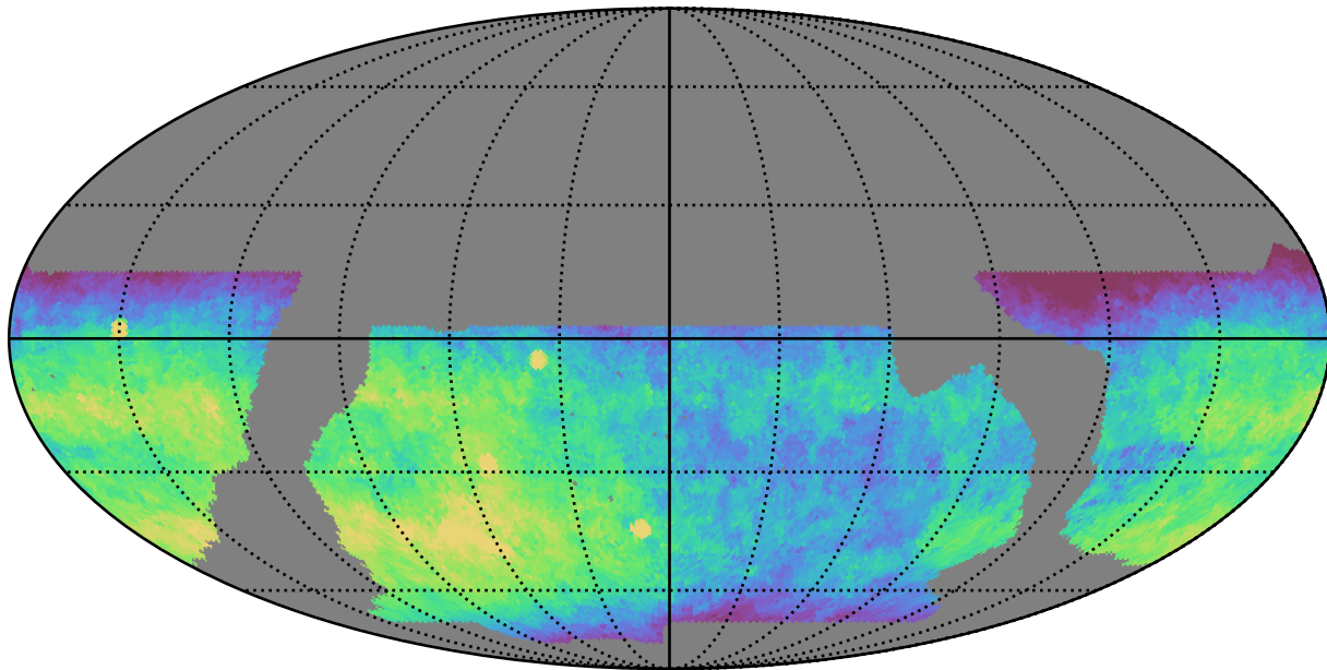
baseline_v2.1_10yrs WFD z band: Median fiveSigmaDepth
