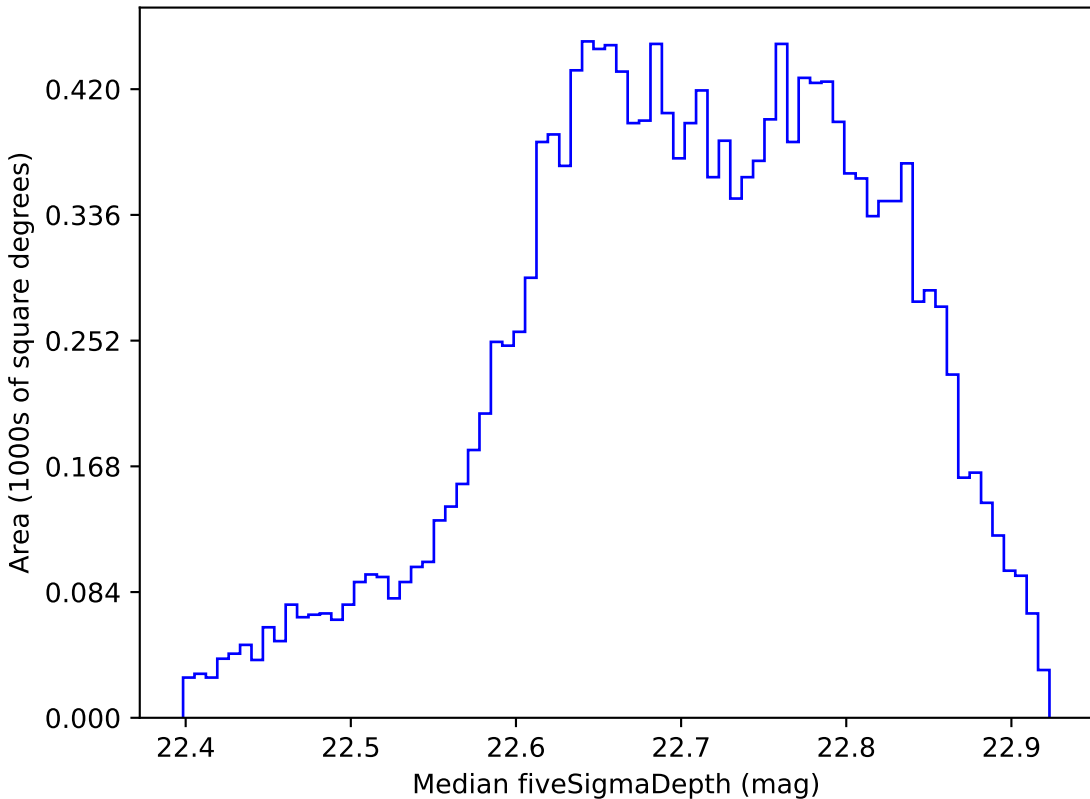
baseline_v2.1_10yrs WFD z band: Median fiveSigmaDepth
